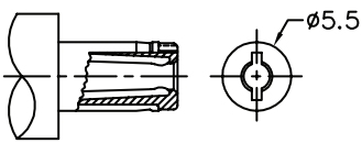
MATING PLUG Jack Insertion Depth: 8.5 mm
