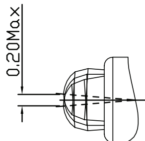
Maximum skewness
