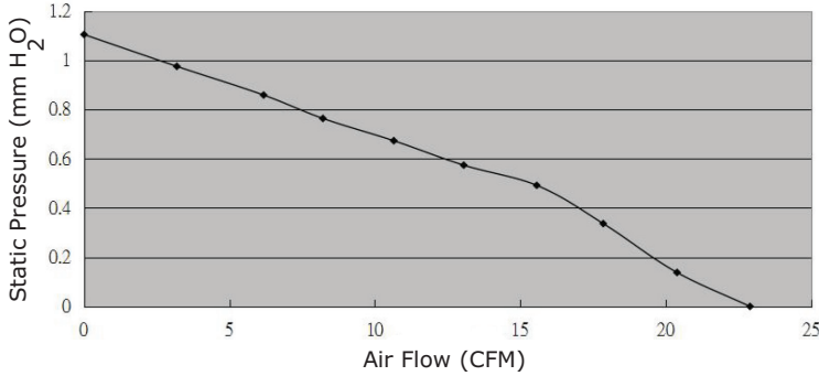
CFM-8015CF-140-363
