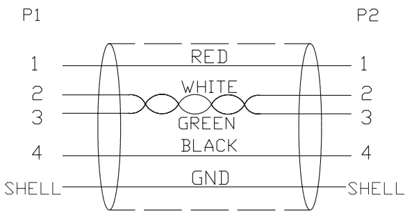
WIRE DIAGRAM
