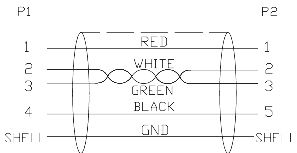
Pin Assignment
